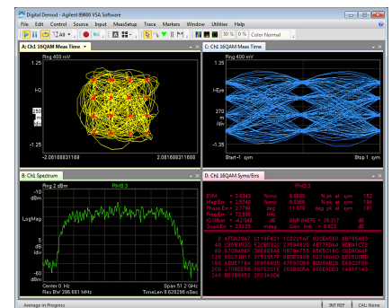
Figure 1. 16QAM @ 32 GBaud.
