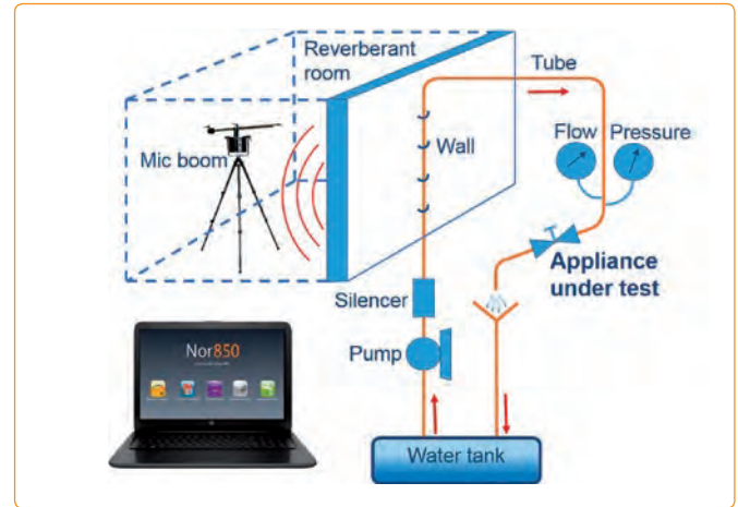
Typical setup of a Appliance Noise test lab
