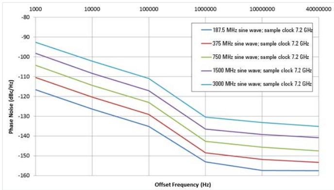
Phase noise plot with internal sample clock, 7.2 GSa/s, direct output measured with balun.
