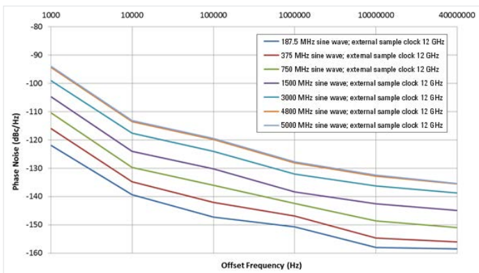
Phase noise plot with external sample clock, 12 GSa/s, direct output measured with balun.
