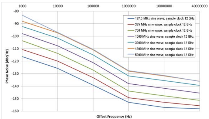
Phase noise plot with internal sample clock, 12 GSa/s, direct output measured with balun.
