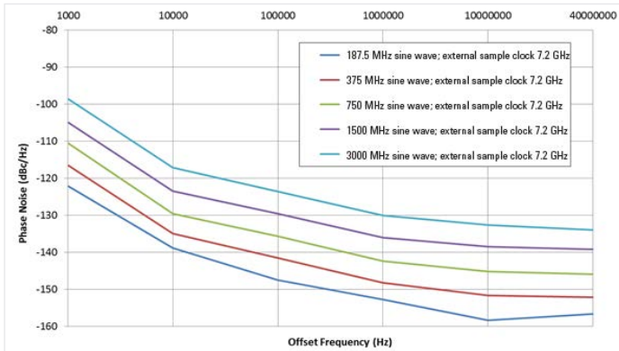
Phase noise plot with external sample clock, 7.2 GSa/s, direct output measured with balun.
