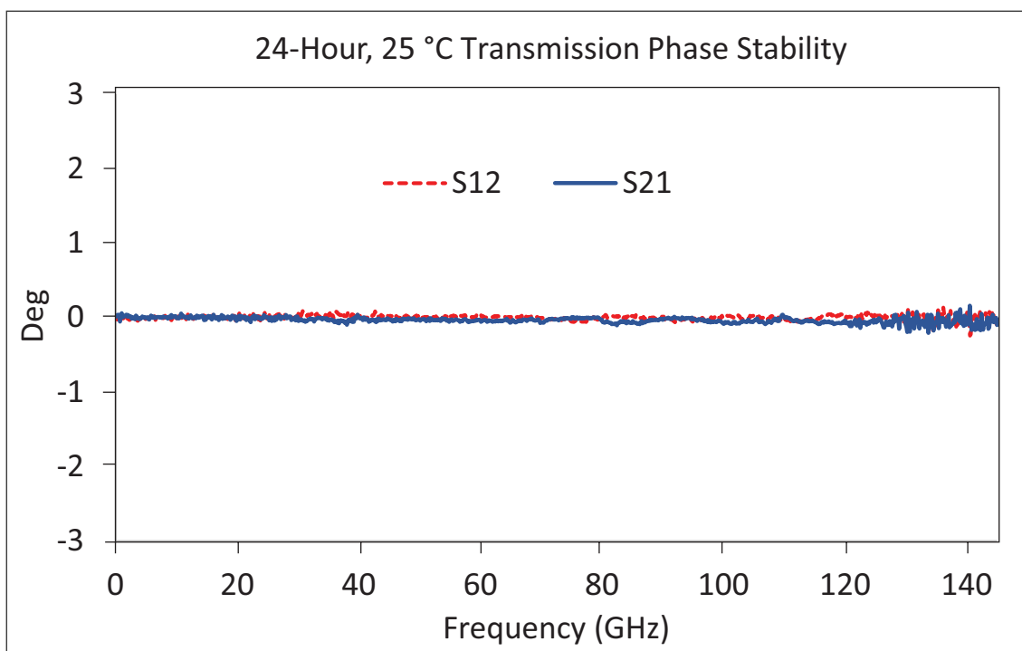
Example 24 Hour Transmission Phase Stability
