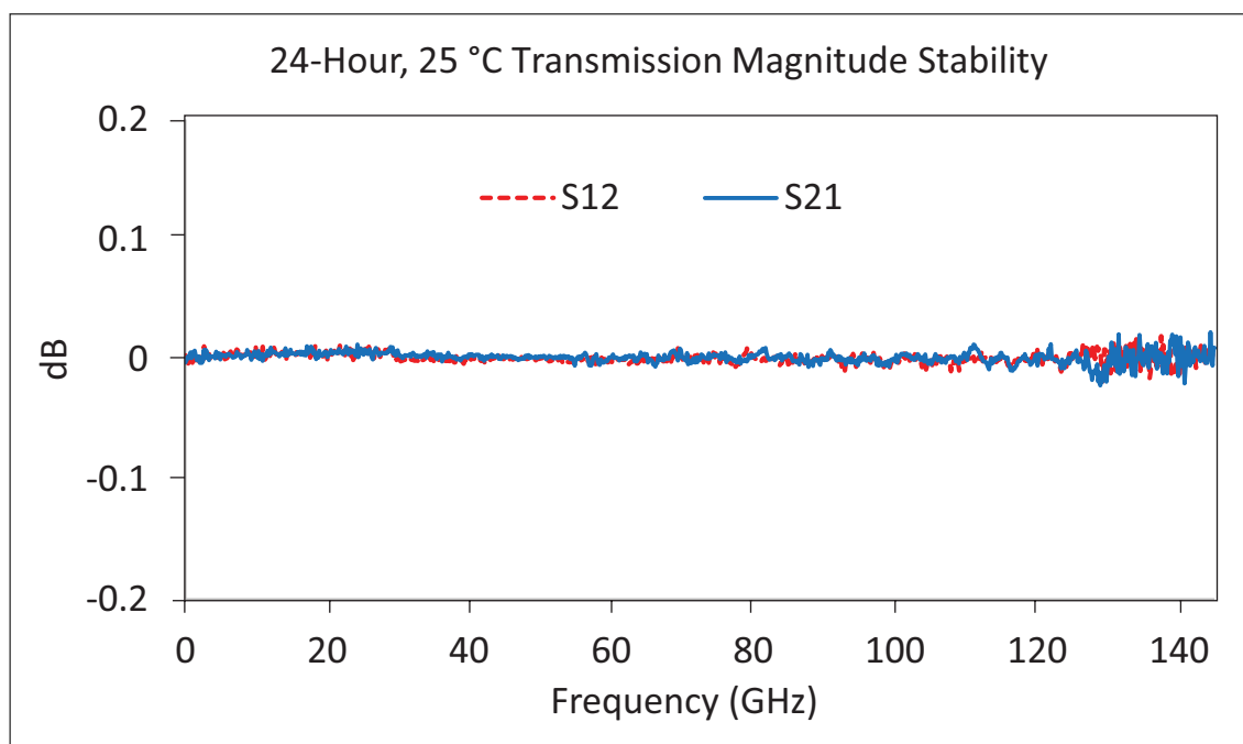
Example 24 Hour Transmission Magnitude Stability
