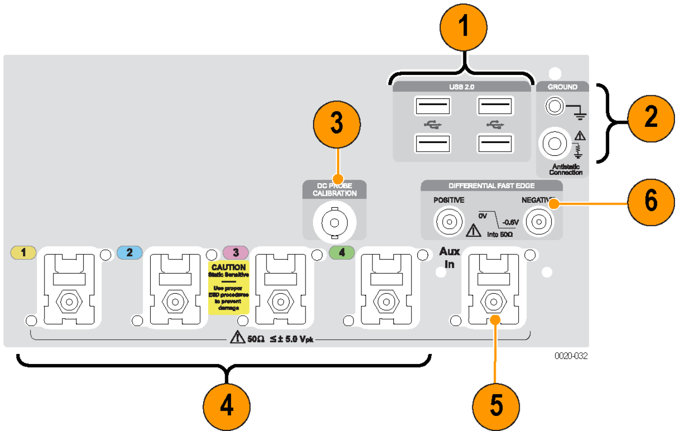
Figure 6: TekConnect channels
