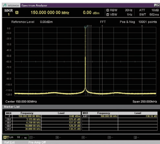
Spectrum Display 150 MHz Measurement Frequency, Preamp Off
