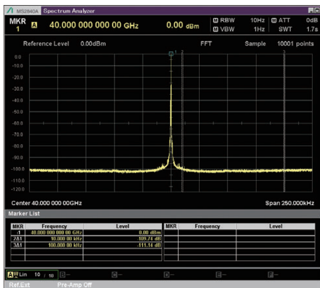
Spectrum Display 40 GHz Measurement Frequency, Preamp Off
