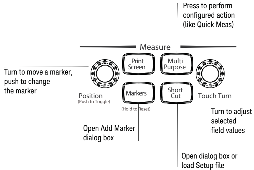
Figure 19 Measure controls
