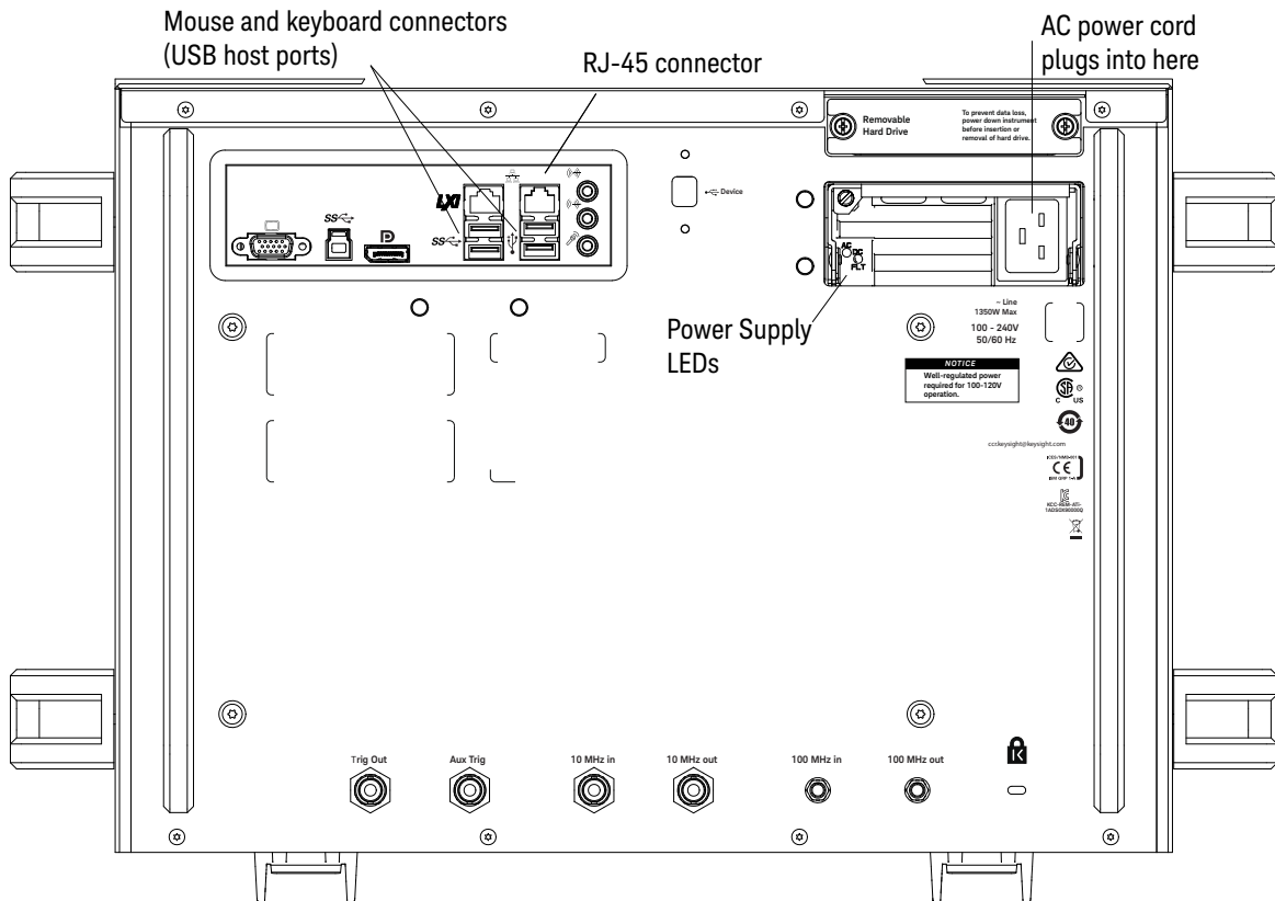
Figure 2 Back panel
