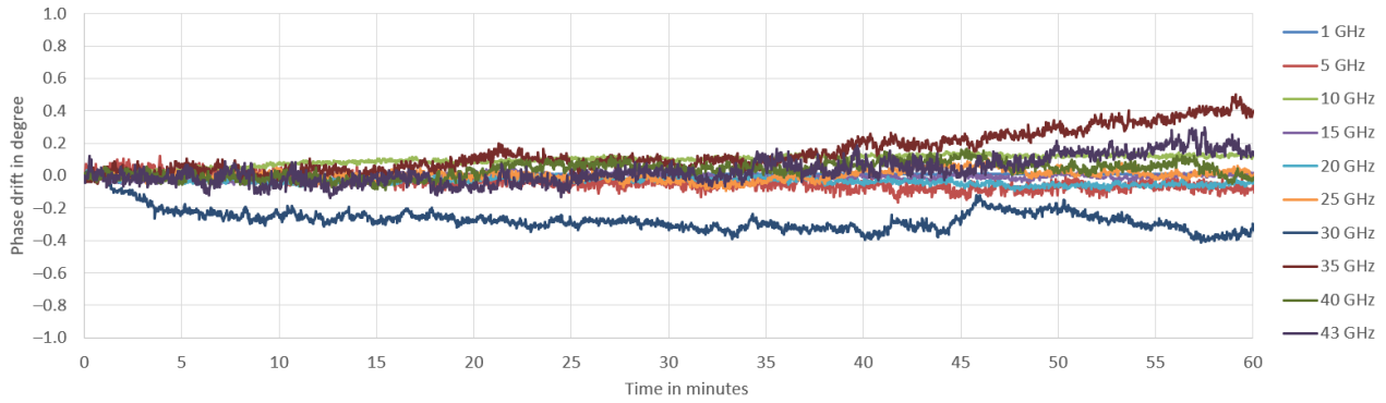
Measured phase drift between RF channels versus time for different RF frequencies
