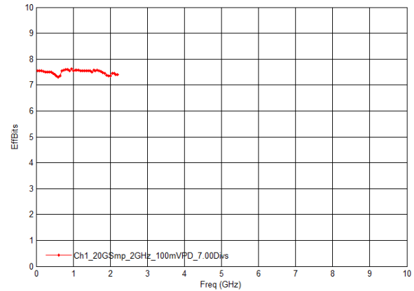
ENOB plot for 2 GHz DSOS204A oscilloscope
