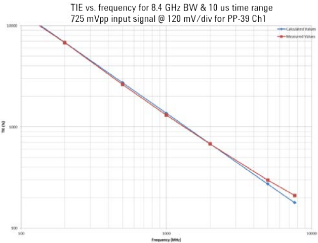
Figure 13. Oscilloscope vendors characterize jitter measurement floor of an oscilloscope by plotting TIE measurements vs input signal slew rate (can also use frequency if sine waves are used). All oscilloscopes in the world except the Infiniium S-Series have an intrinsic jitter plot that resembles the one on the left. The plot shows that intrinsic jitter values are dominated by slew rate and vertical noise until the horizontal system becomes the biggest contributor. This is known as the jitter measurement floor. The impressive S-Series jitter curve is a function of vertical noise and slew rate--meaning that the oscilloscope's horizontal system is a non-contributor to overall intrinsic jitter. Infiniium S-Series has in-band intrinsic jitter of under 120 fs for input sine waves of 8 GHz (max BW).
