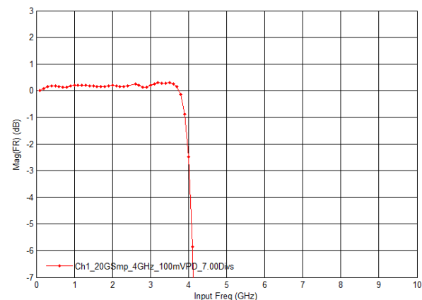
Magnitude response for 4 GHz DSOS404A oscilloscope
