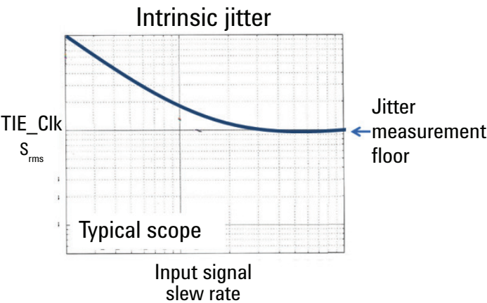
Figure 13. Oscilloscope vendors characterize jitter measurement floor of an oscilloscope by plotting TIE measurements vs input signal slew rate (can also use frequency if sine waves are used). All oscilloscopes in the world except the Infiniium S-Series have an intrinsic jitter plot that resembles the one on the left. The plot shows that intrinsic jitter values are dominated by slew rate and vertical noise until the horizontal system becomes the biggest contributor. This is known as the jitter measurement floor. The impressive S-Series jitter curve is a function of vertical noise and slew rate--meaning that the oscilloscope's horizontal system is a non-contributor to overall intrinsic jitter. Infiniium S-Series has in-band intrinsic jitter of under 120 fs for input sine waves of 8 GHz (max BW).
