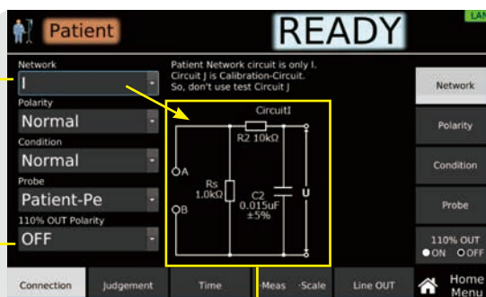
Measurement circuit network (network I IEC60601-1)
